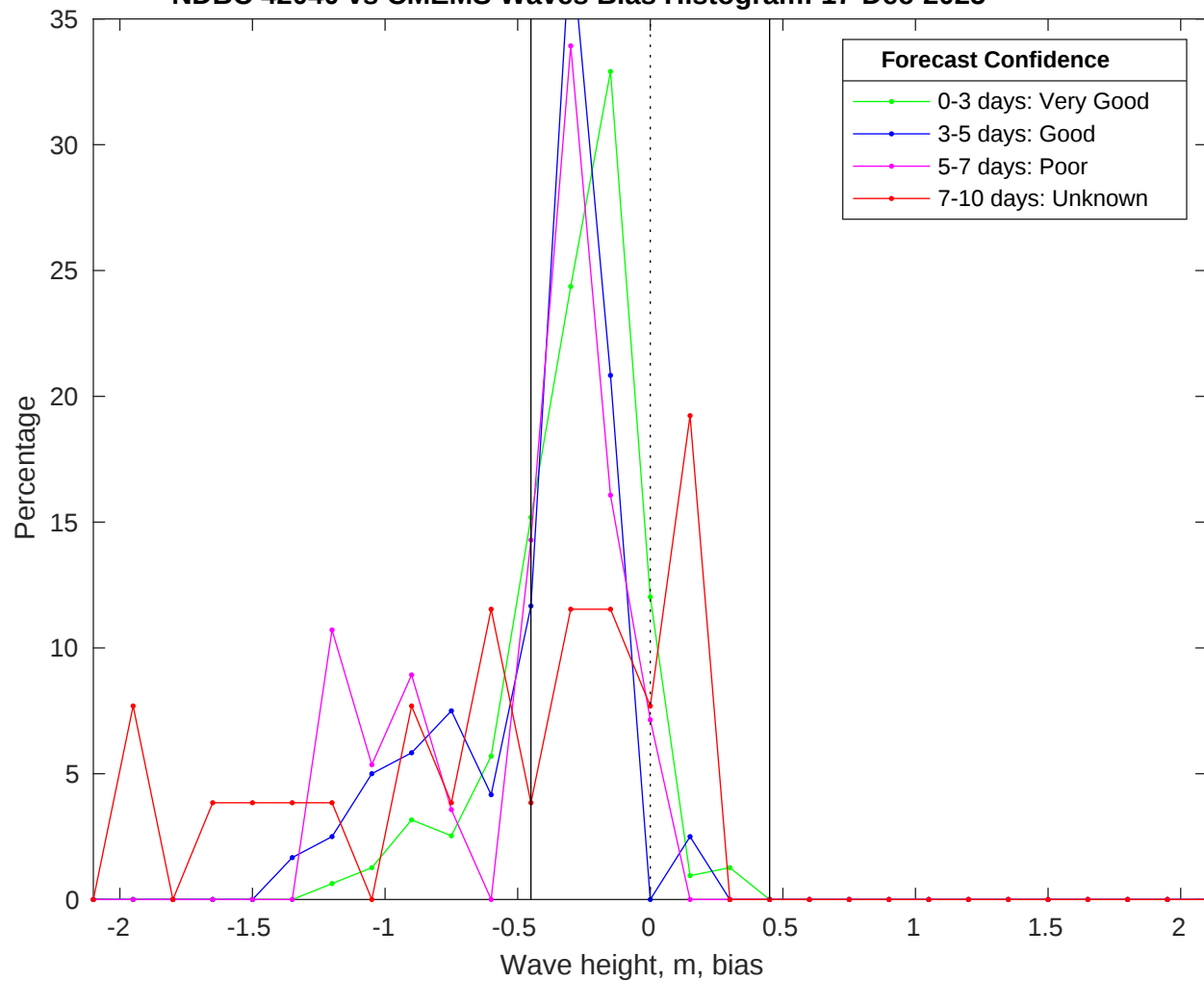
NDBC 42040 vs CMEMS Waves Bias Histogram: 17-Dec-2025
