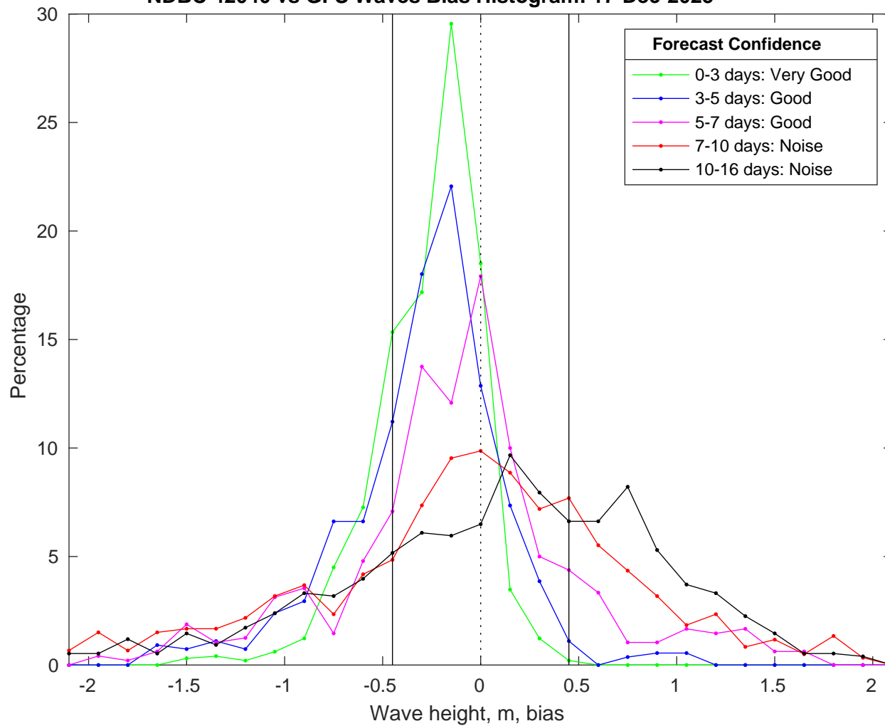
NDBC 42040 vs GFS Waves Bias Histogram: 17-Dec-2025
