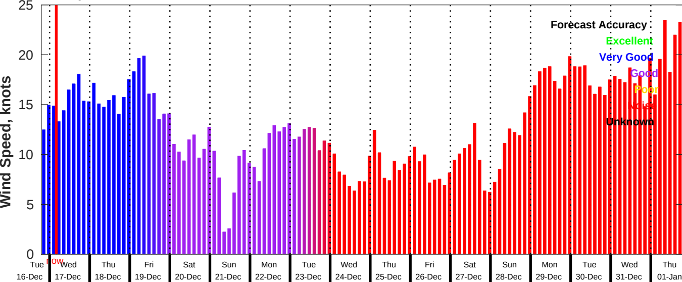
GFS Wind Speed Forecast for NDBC 42040 from 16-Dec-2025 19:00:00 to 01-Jan-2026 19:00:00
