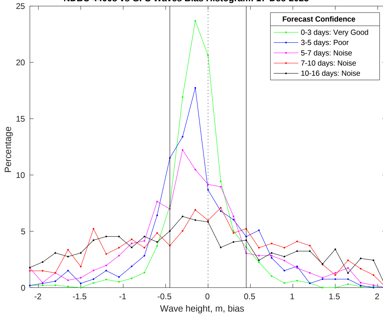
NDBC 44008 vs GFS Waves Bias Histogram: 17-Dec-2025
