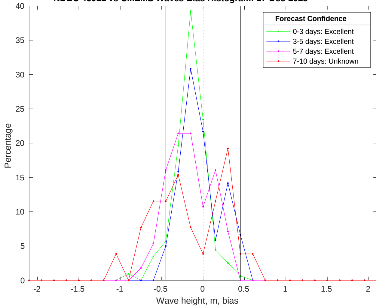
NDBC 46011 vs CMEMS Waves Bias Histogram: 17-Dec-2025
