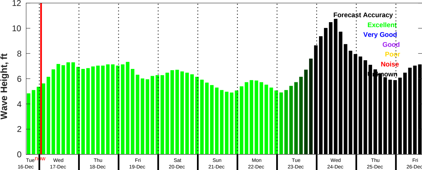
CMEMS Wave Forecast for NDBC 46011 from 16-Dec-2025 16:00:00 to 26-Dec-2025 16:00:00
