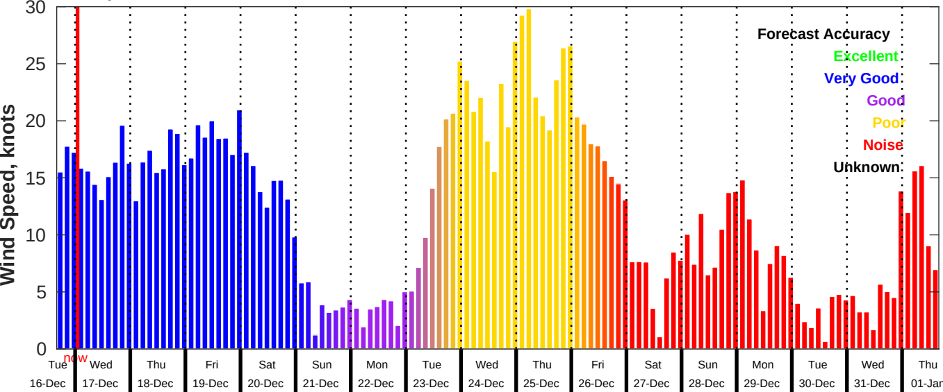
GFS Wind Speed Forecast for NDBC 46011 from 16-Dec-2025 16:00:00 to 01-Jan-2026 16:00:00
