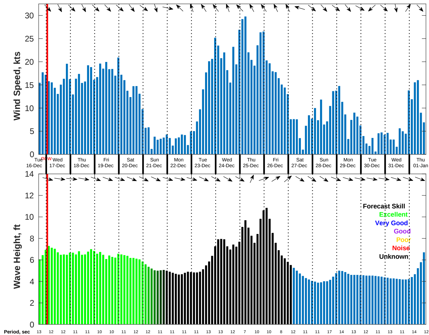
Wind & Wave Forecast for NDBC 46011 from 16-Dec-2025 16:00:00 to 01-Jan-2026 16:00:00
