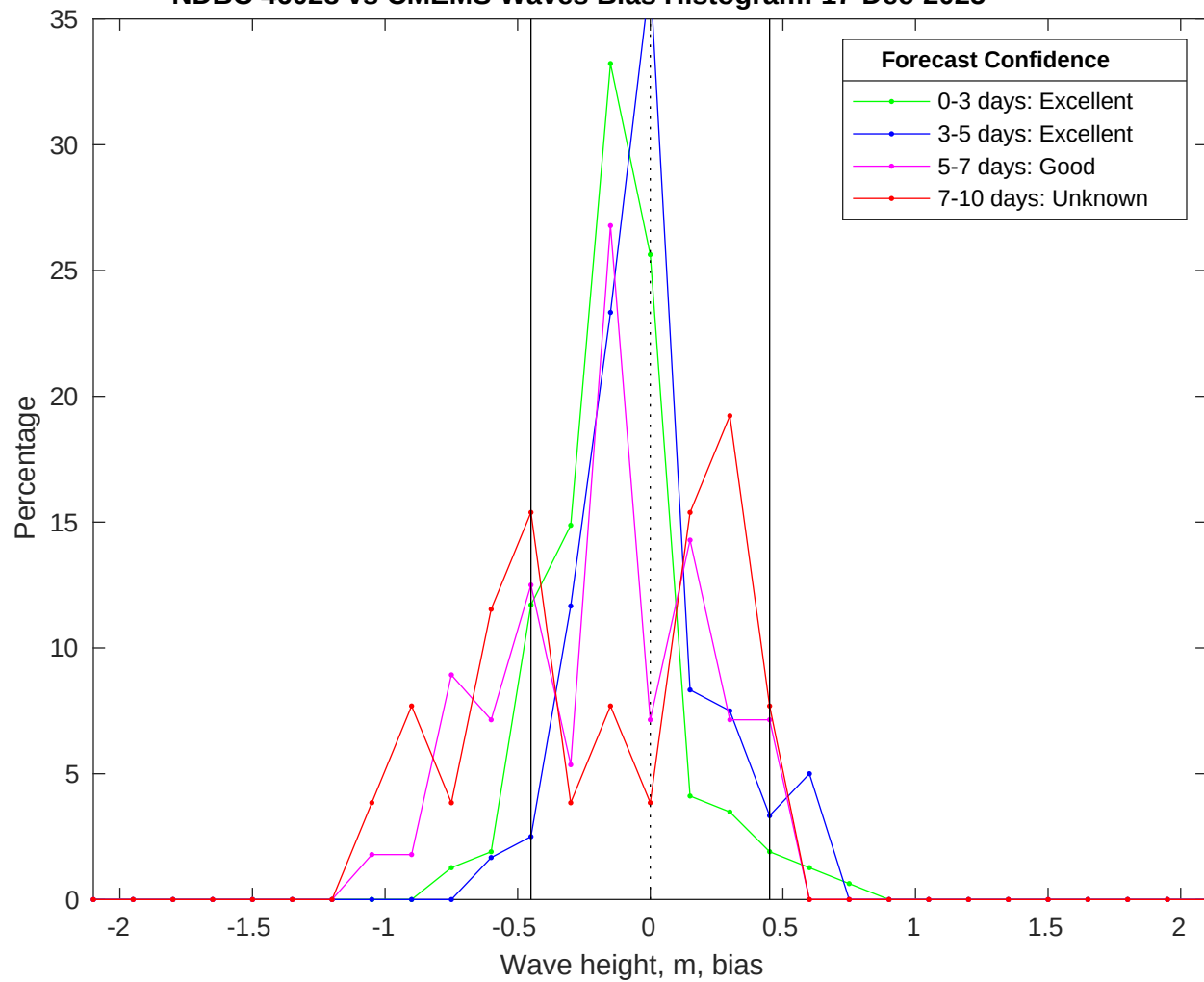
NDBC 46028 vs CMEMS Waves Bias Histogram: 17-Dec-2025
