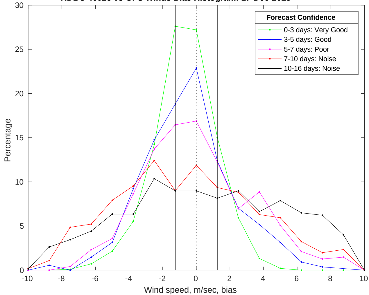
NDBC 46028 vs GFS Winds Bias Histogram: 17-Dec-2025
