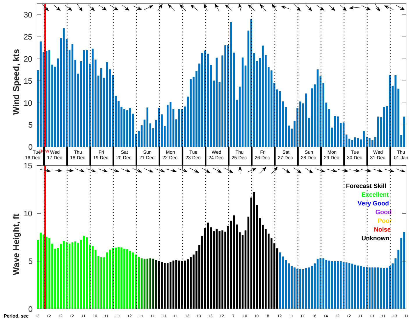
Wind & Wave Forecast for NDBC 46028 from 16-Dec-2025 16:00:00 to 01-Jan-2026 16:00:00
