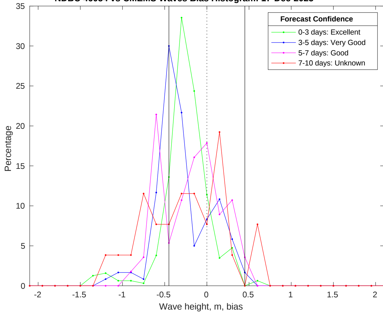
NDBC 46054 vs CMEMS Waves Bias Histogram: 17-Dec-2025
