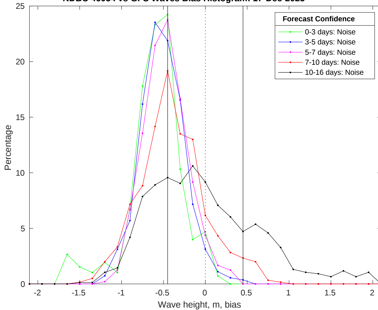
NDBC 46054 vs GFS Waves Bias Histogram: 17-Dec-2025
