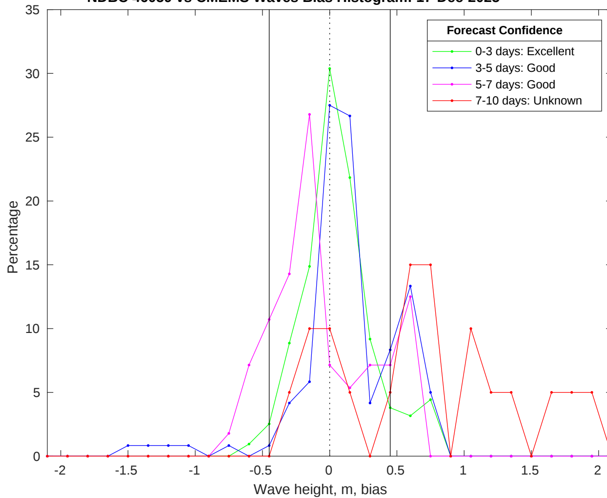
NDBC 46059 vs CMEMS Waves Bias Histogram: 17-Dec-2025
