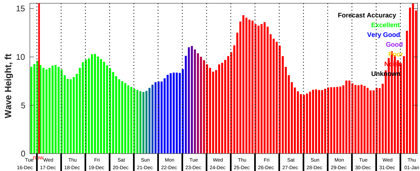
GFS Wave Forecast for NDBC 46059 from 16-Dec-2025 17:00:00 to 01-Jan-2026 17:00:00
