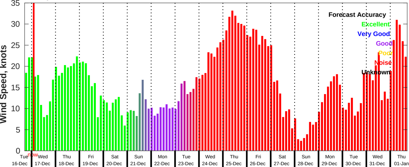
GFS Wind Speed Forecast for NDBC 46059 from 16-Dec-2025 17:00:00 to 01-Jan-2026 17:00:00
