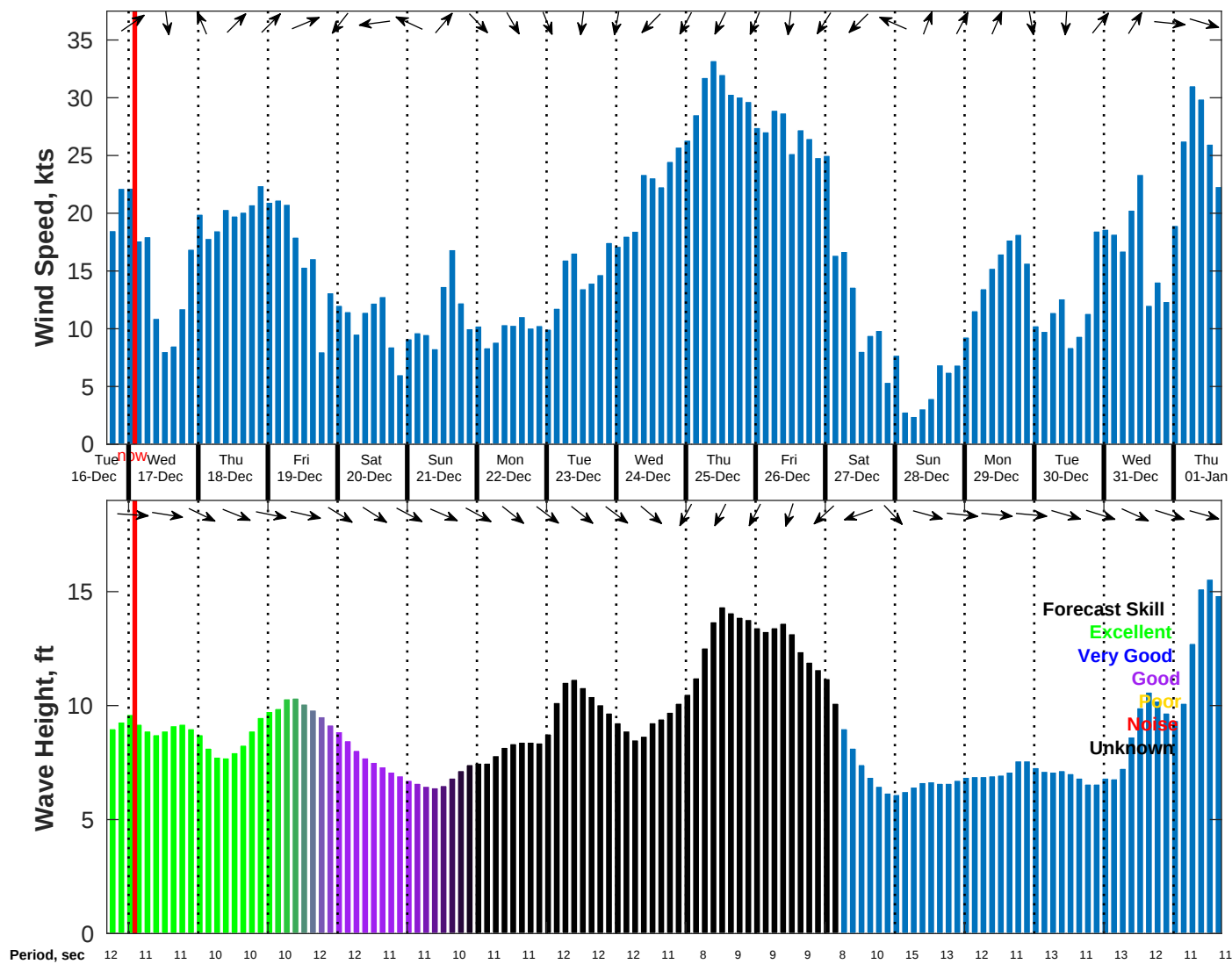
Wind & Wave Forecast for NDBC 46059 from 16-Dec-2025 17:00:00 to 01-Jan-2026 17:00:00
