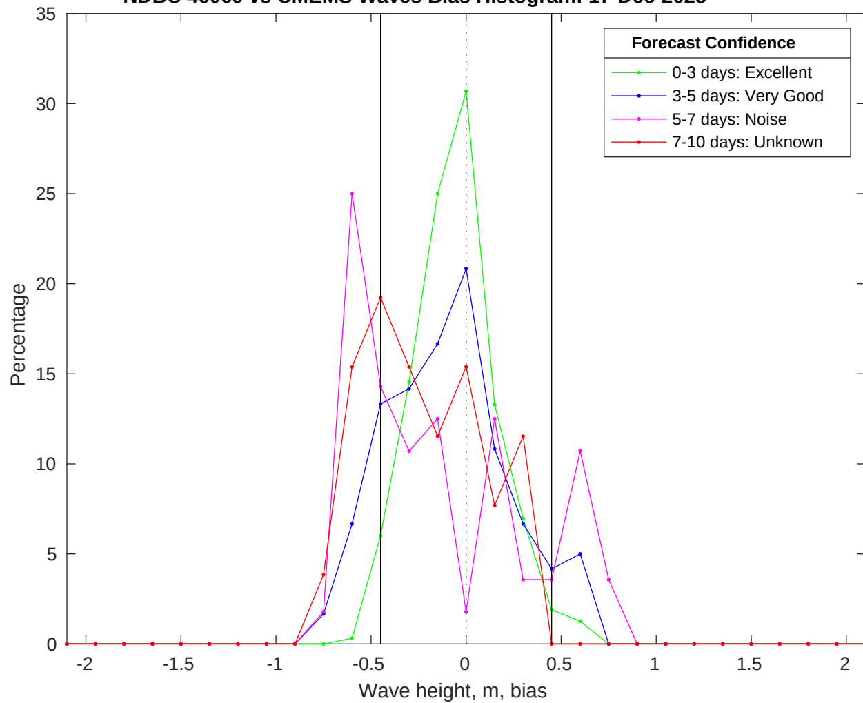
NDBC 46069 vs CMEMS Waves Bias Histogram: 17-Dec-2025
