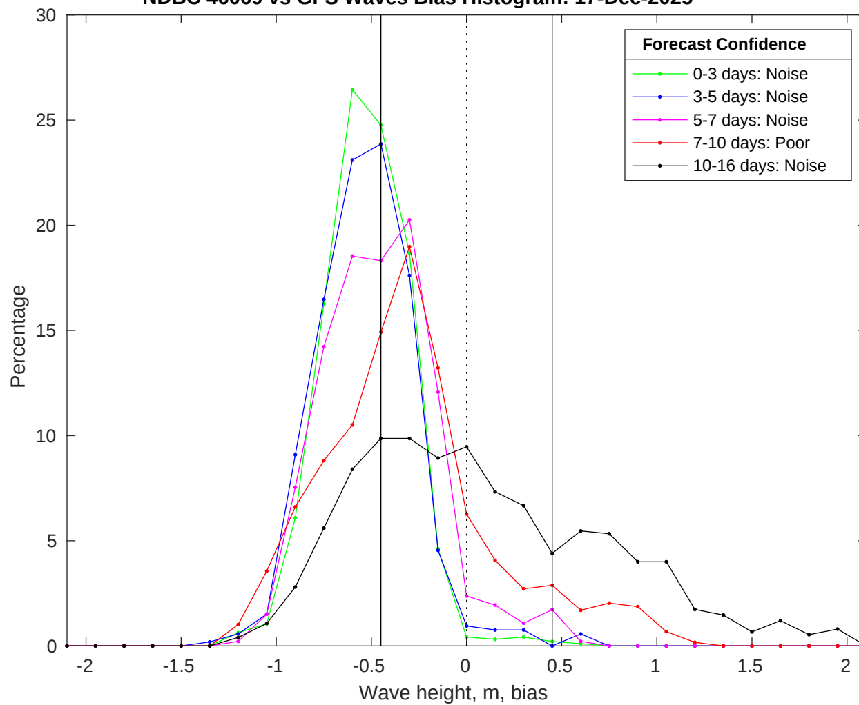
NDBC 46069 vs GFS Waves Bias Histogram: 17-Dec-2025
