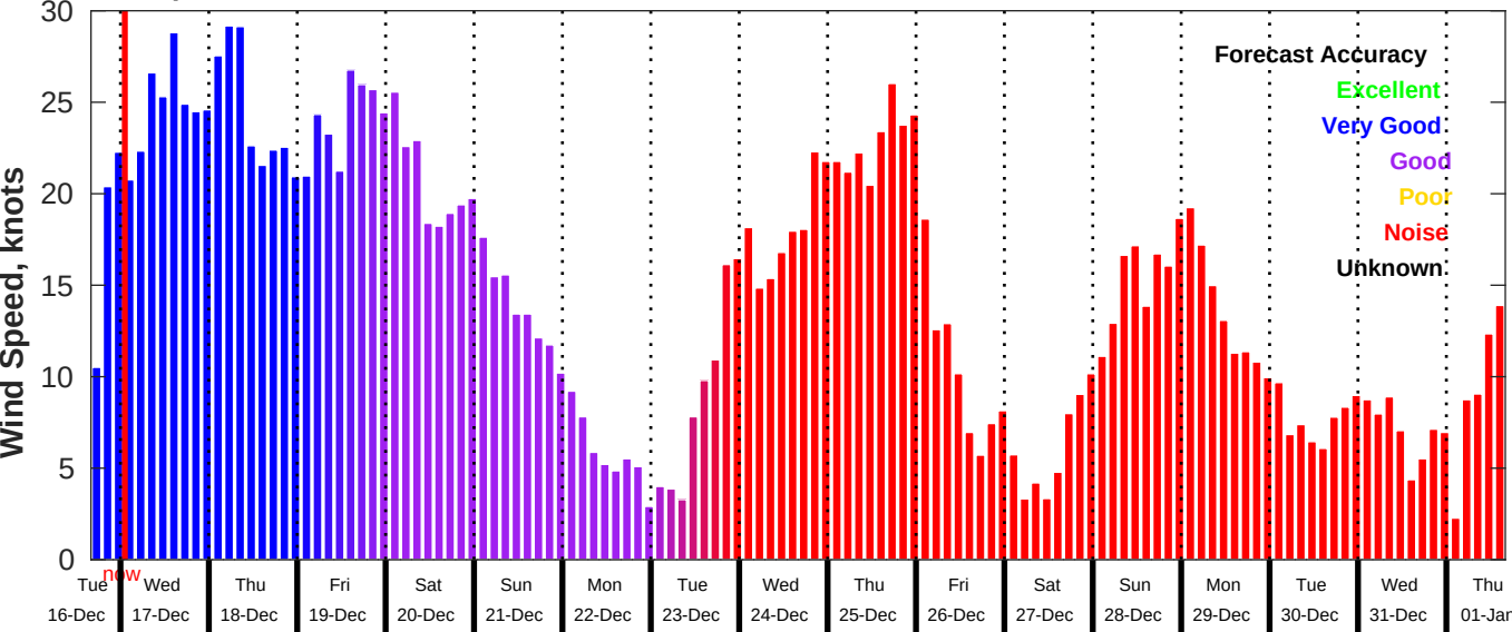
GFS Wind Speed Forecast for NDBC 46069 from 16-Dec-2025 16:00:00 to 01-Jan-2026 16:00:00
