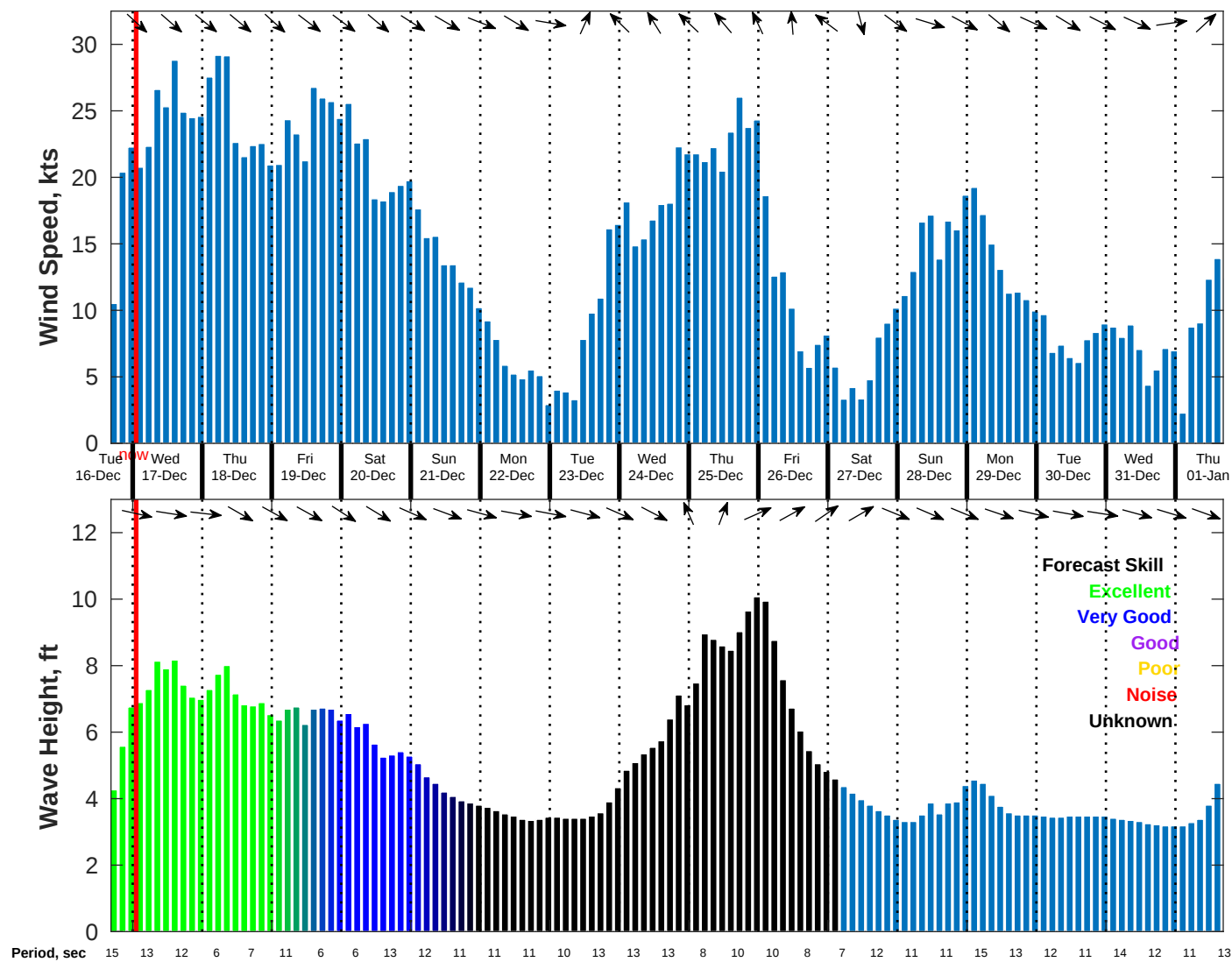
Wind & Wave Forecast for NDBC 46069 from 16-Dec-2025 16:00:00 to 01-Jan-2026 16:00:00
