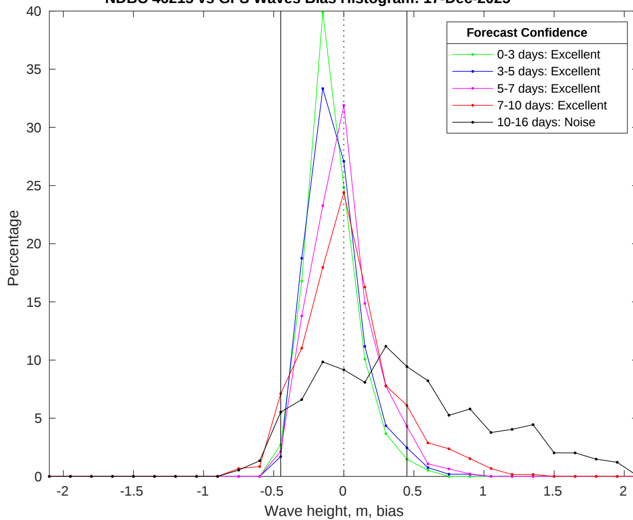
NDBC 46215 vs GFS Waves Bias Histogram: 17-Dec-2025
