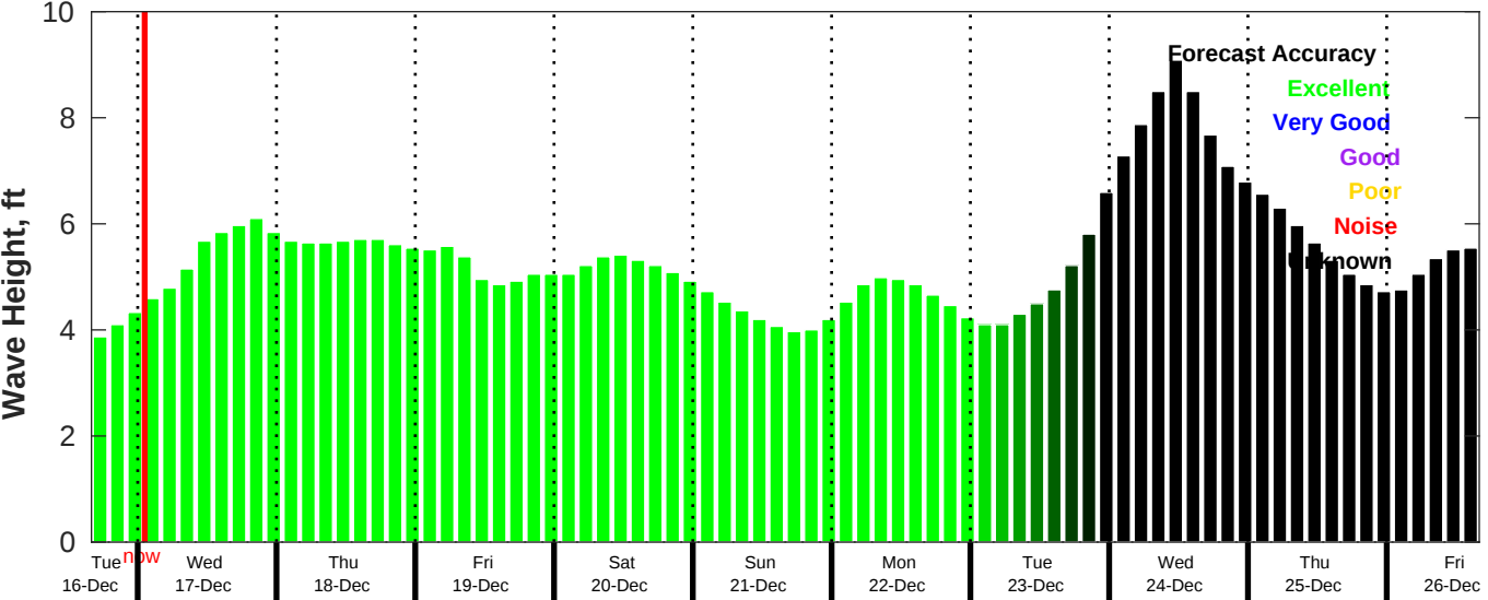
CMEMS Wave Forecast for NDBC 46215 from 16-Dec-2025 16:00:00 to 26-Dec-2025 16:00:00
