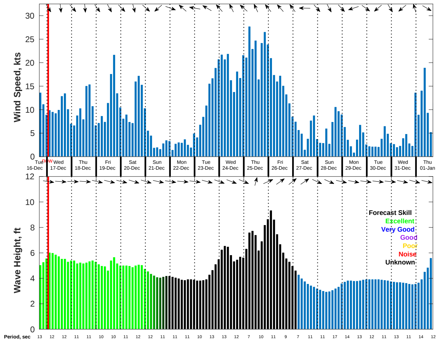
Wind & Wave Forecast for NDBC 46215 from 16-Dec-2025 16:00:00 to 01-Jan-2026 16:00:00
