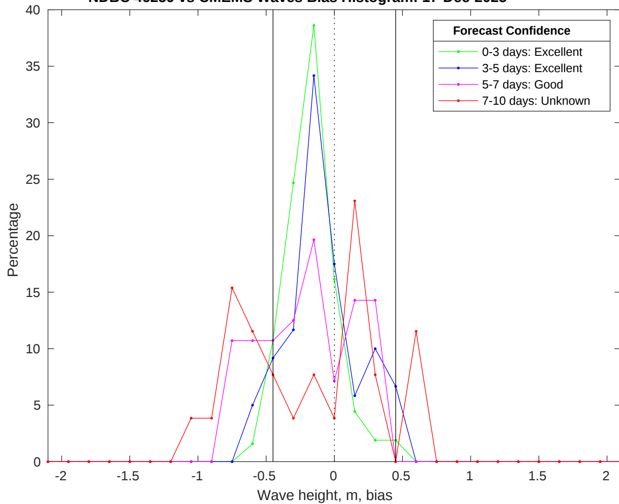
NDBC 46259 vs CMEMS Waves Bias Histogram: 17-Dec-2025
