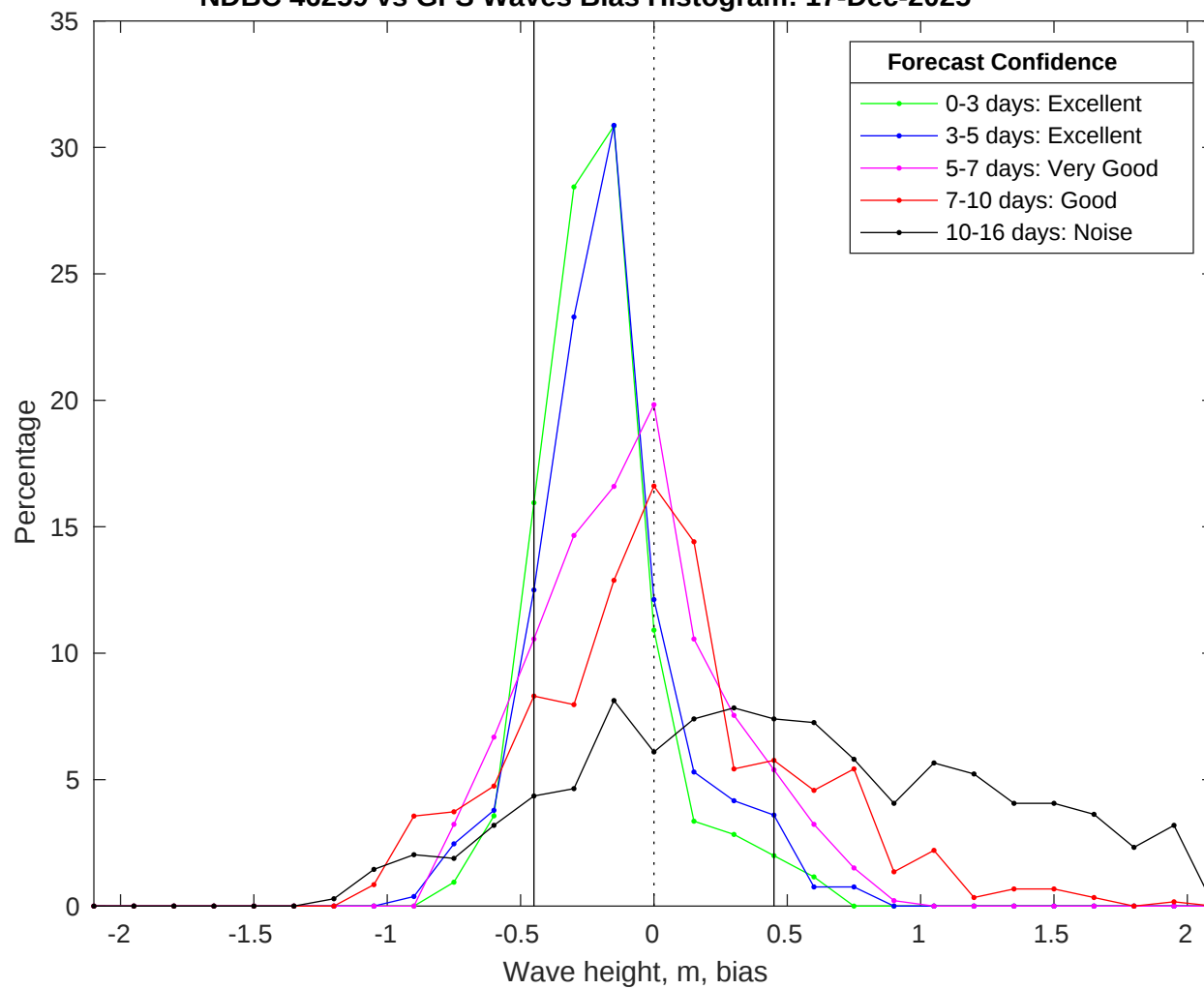
NDBC 46259 vs GFS Waves Bias Histogram: 17-Dec-2025
