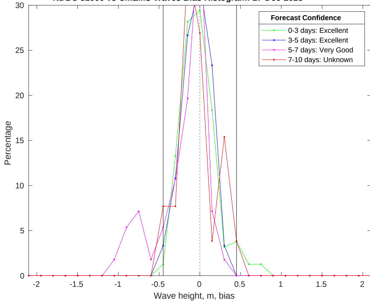
NDBC 51000 vs CMEMS Waves Bias Histogram: 17-Dec-2025
