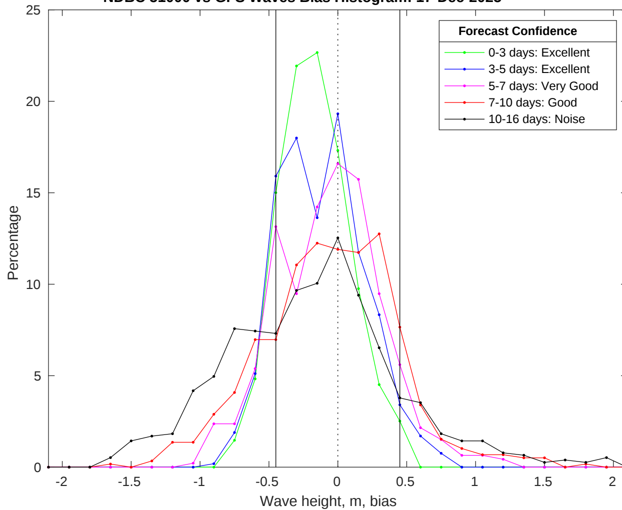
NDBC 51000 vs GFS Waves Bias Histogram: 17-Dec-2025
