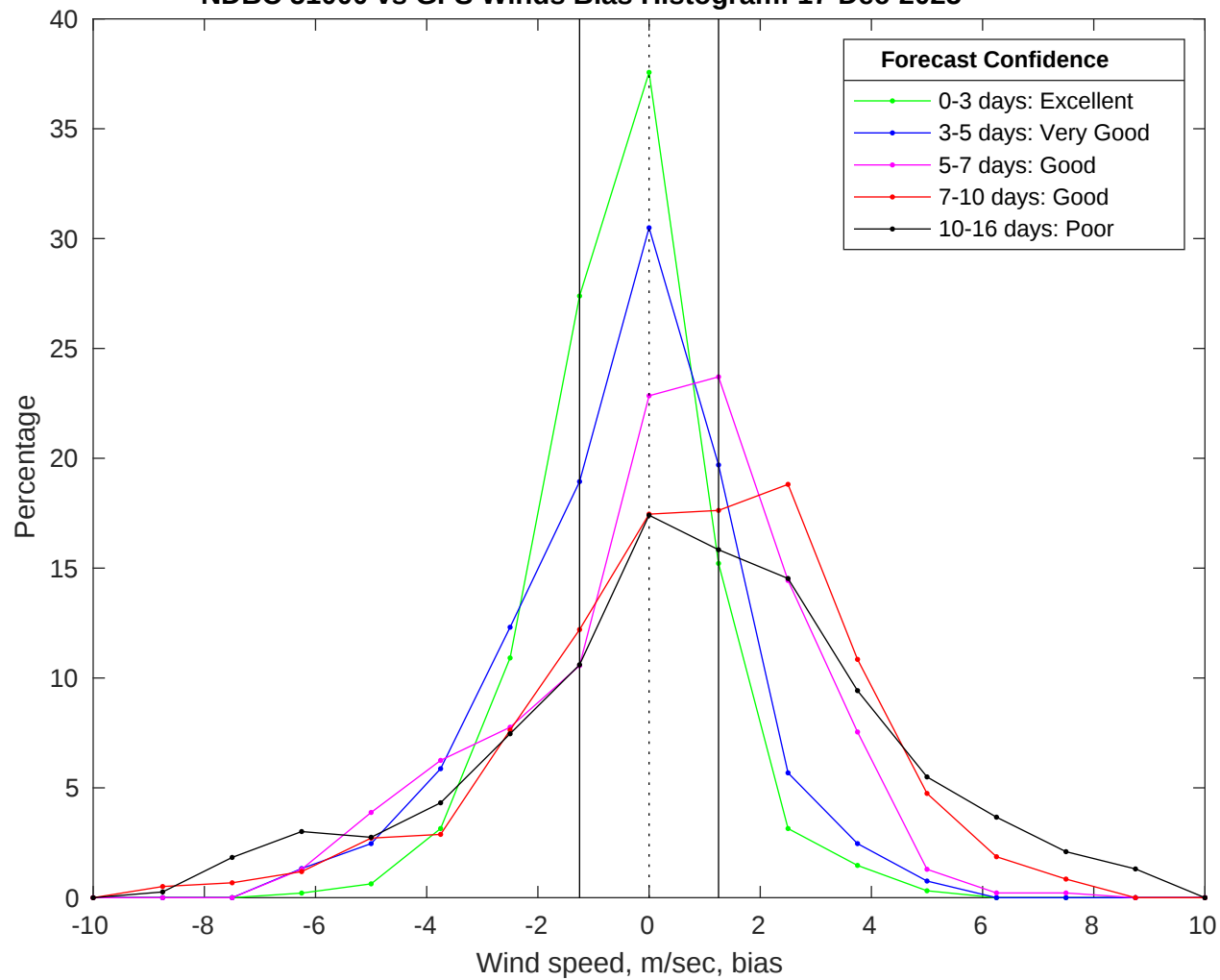
NDBC 51000 vs GFS Winds Bias Histogram: 17-Dec-2025
