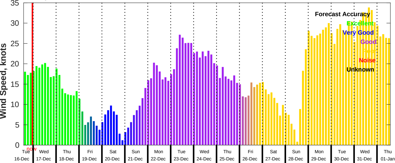
GFS Wind Speed Forecast for NDBC 51000 from 16-Dec-2025 14:00:00 to 01-Jan-2026 14:00:00
