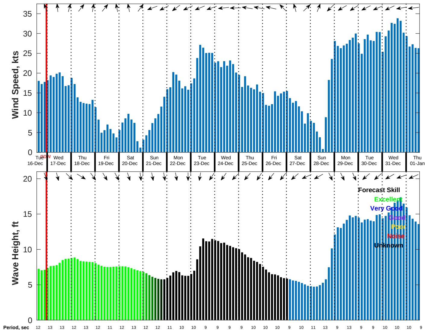
Wind & Wave Forecast for NDBC 51000 from 16-Dec-2025 14:00:00 to 01-Jan-2026 14:00:00
