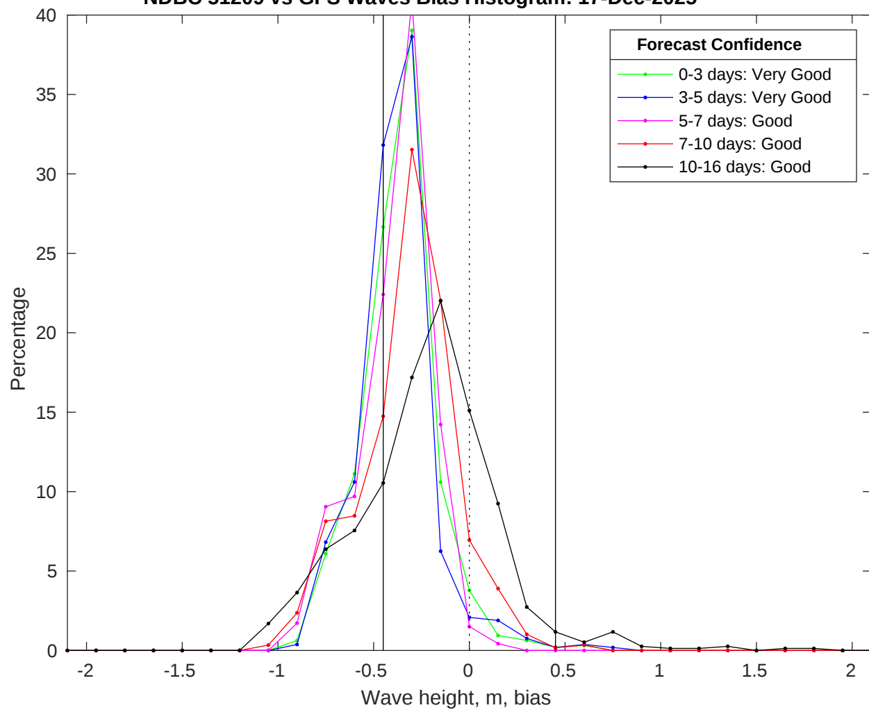
NDBC 51209 vs GFS Waves Bias Histogram: 17-Dec-2025
