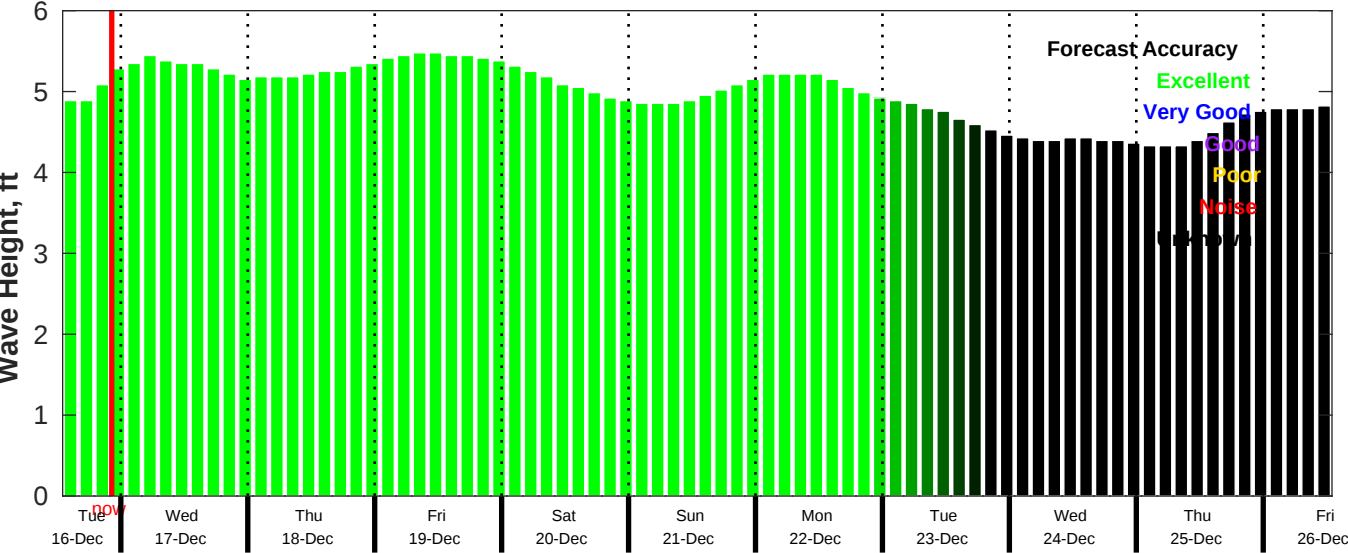
CMEMS Wave Forecast for NDBC 51209 from 16-Dec-2025 13:00:00 to 26-Dec-2025 13:00:00
