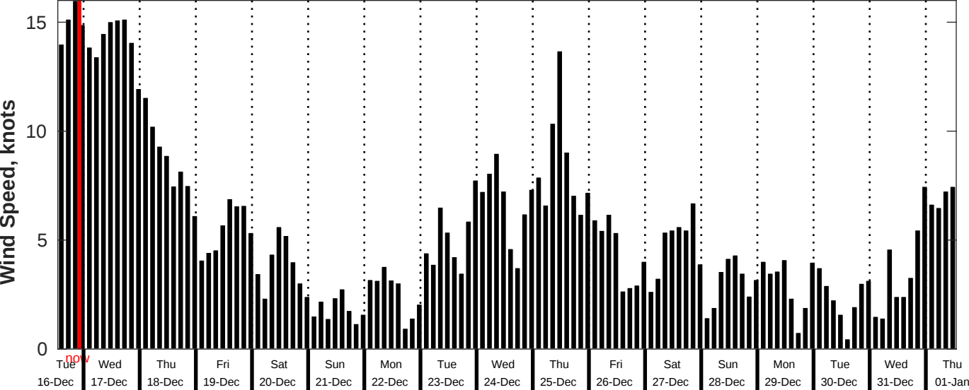
GFS Wind Speed Forecast for NDBC 51209 from 16-Dec-2025 13:00:00 to 01-Jan-2026 13:00:00
