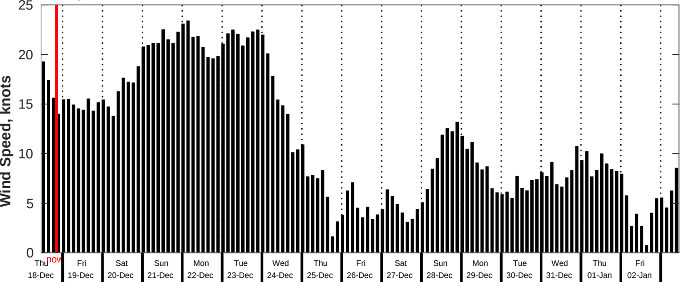
GFS Wind Speed Forecast for NDBC 52211 from 17-Dec-2025 11:00:00 to 02-Jan-2026 11:00:00
