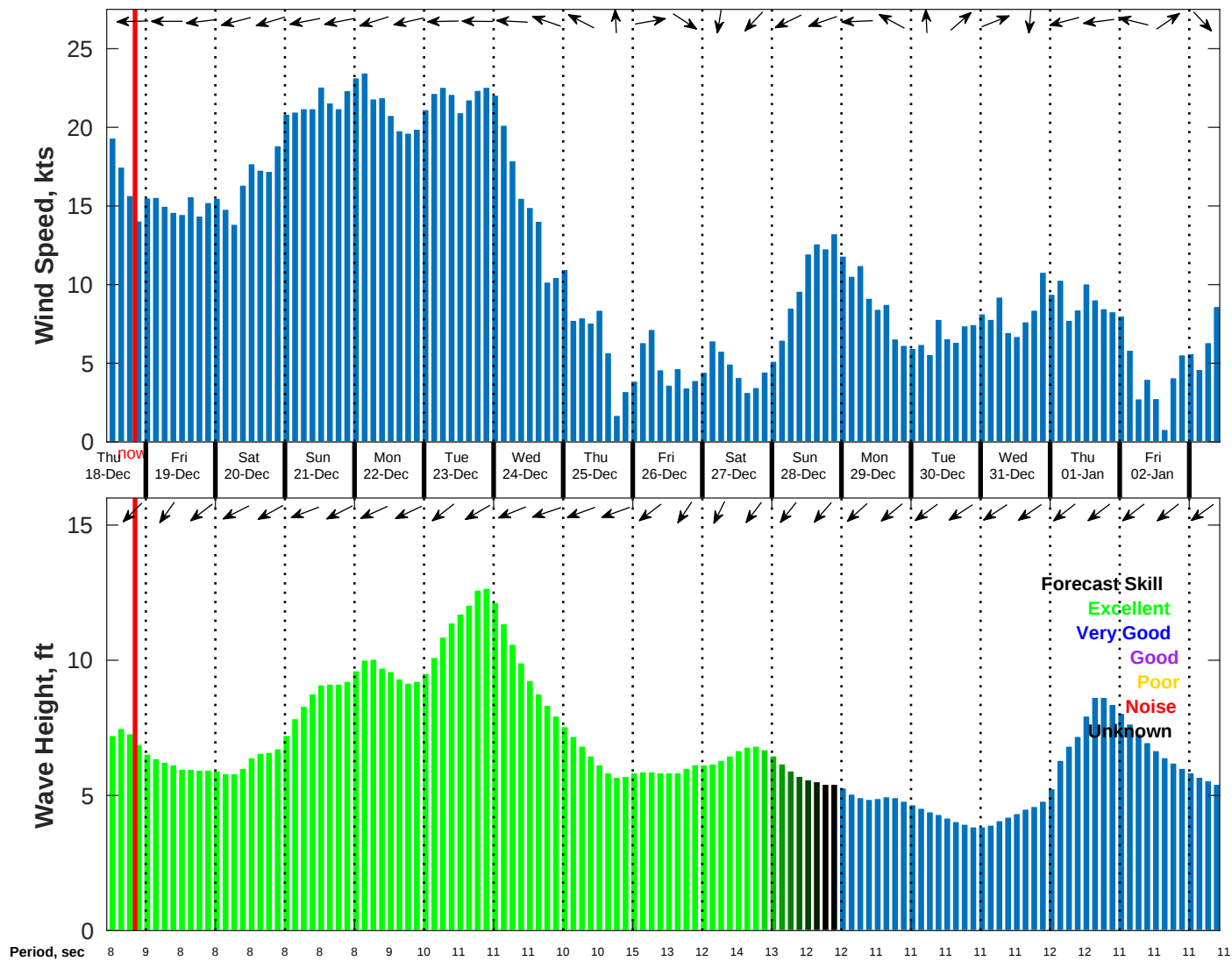
Wind & Wave Forecast for NDBC 52211 from 17-Dec-2025 11:00:00 to 02-Jan-2026 11:00:00
