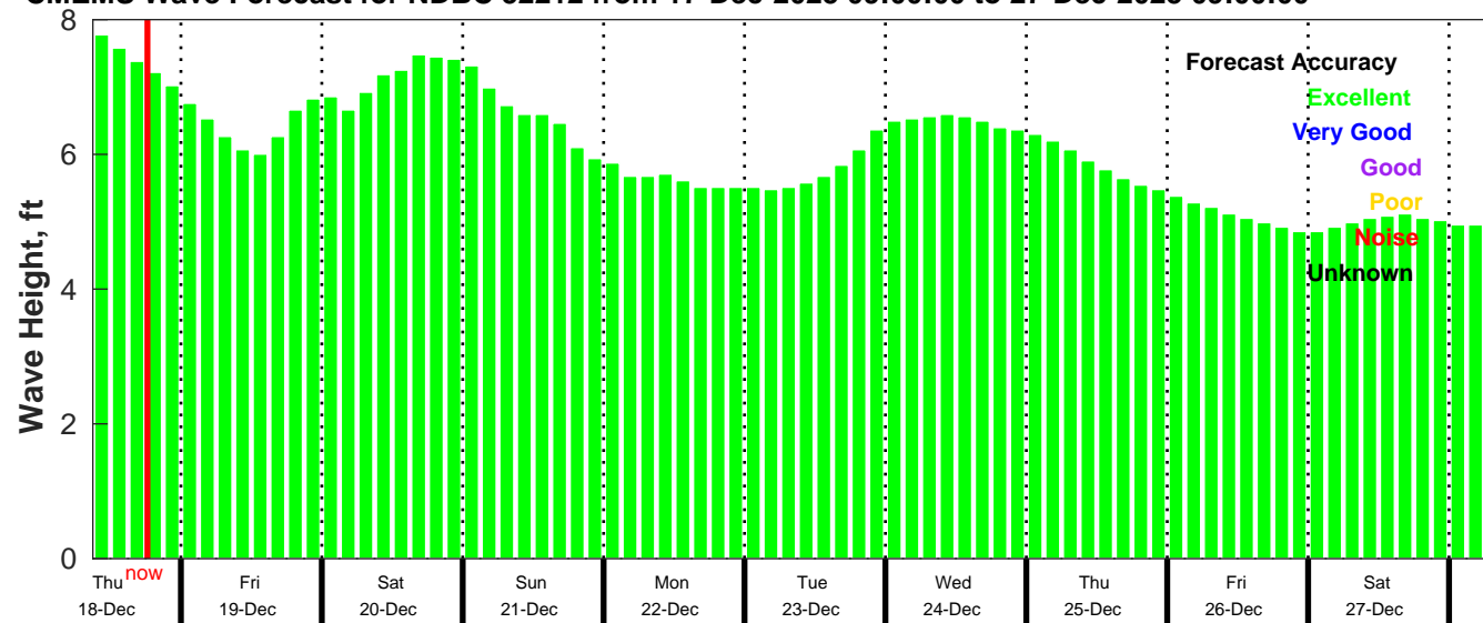
CMEMS Wave Forecast for NDBC 52212 from 17-Dec-2025 09:00:00 to 27-Dec-2025 09:00:00
