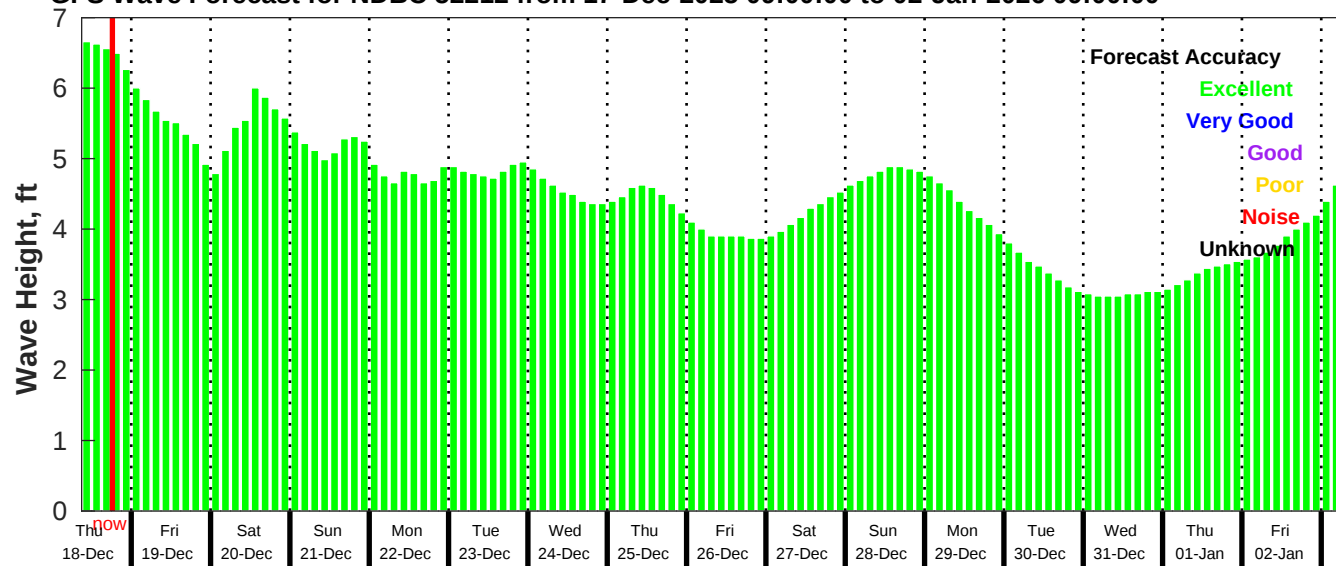
GFS Wave Forecast for NDBC 52212 from 17-Dec-2025 09:00:00 to 02-Jan-2026 09:00:00
