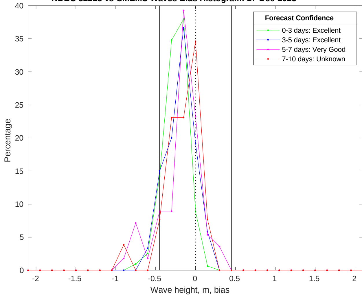
NDBC 52213 vs CMEMS Waves Bias Histogram: 17-Dec-2025
