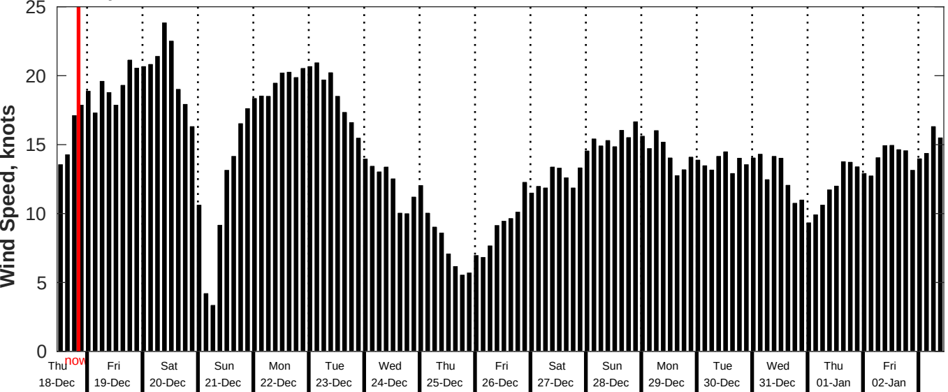
GFS Wind Speed Forecast for NDBC 52213 from 17-Dec-2025 11:00:00 to 02-Jan-2026 11:00:00
