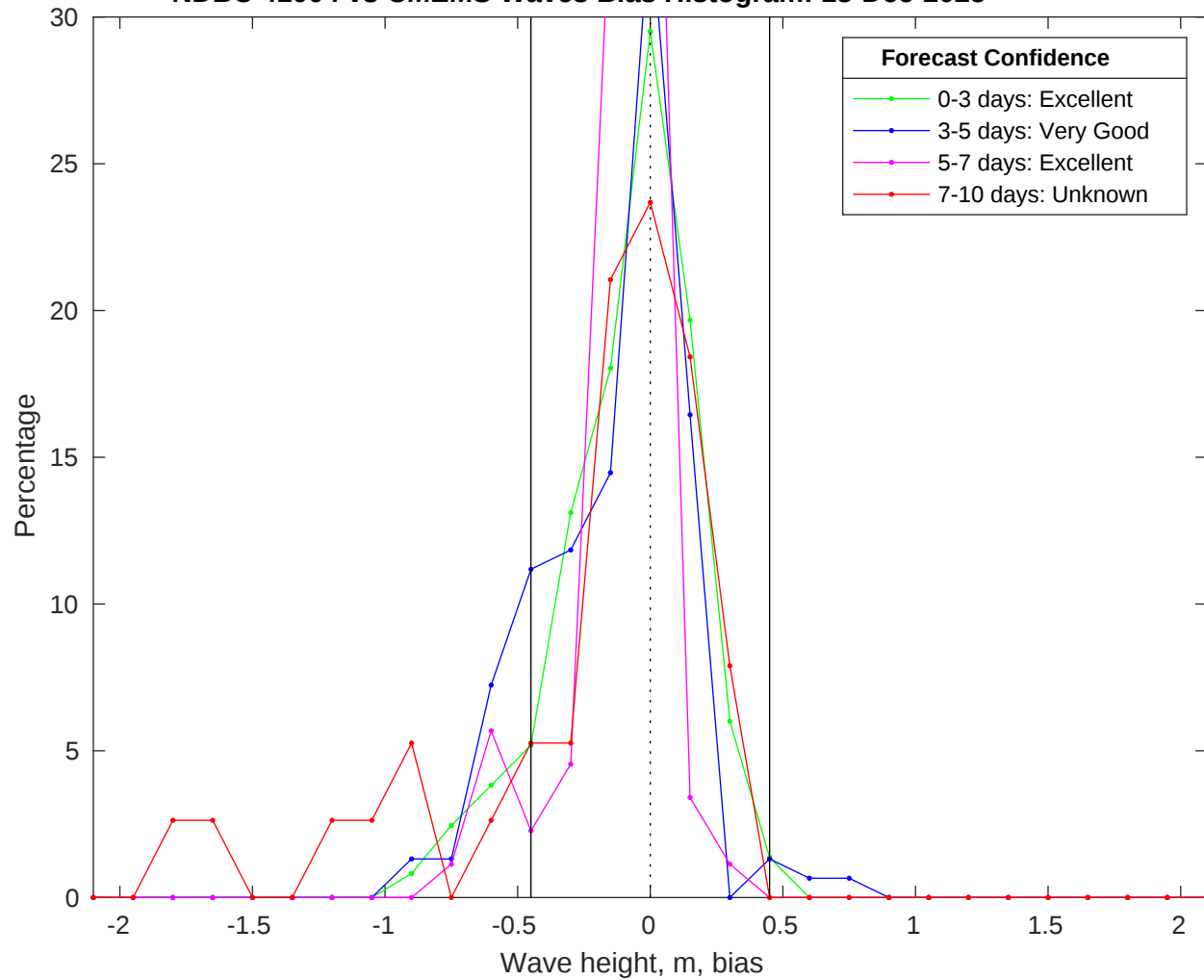
NDBC 41004 vs CMEMS Waves Bias Histogram: 18-Dec-2025
