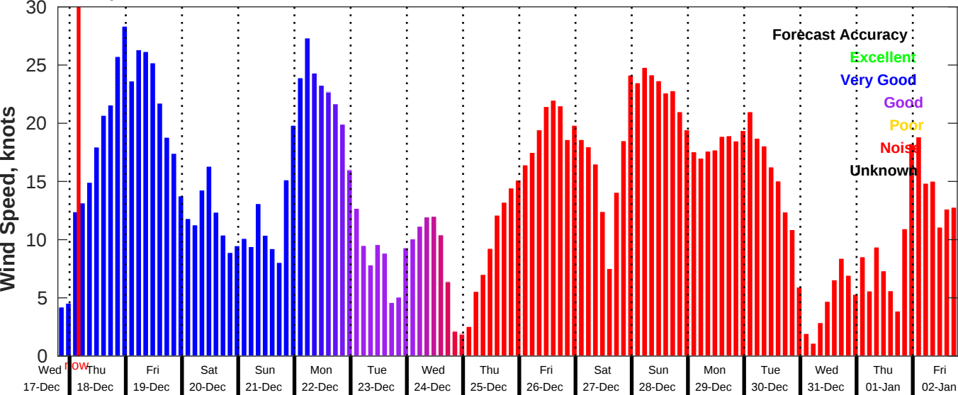
GFS Wind Speed Forecast for NDBC 41004 from 17-Dec-2025 19:00:00 to 02-Jan-2026 19:00:00
