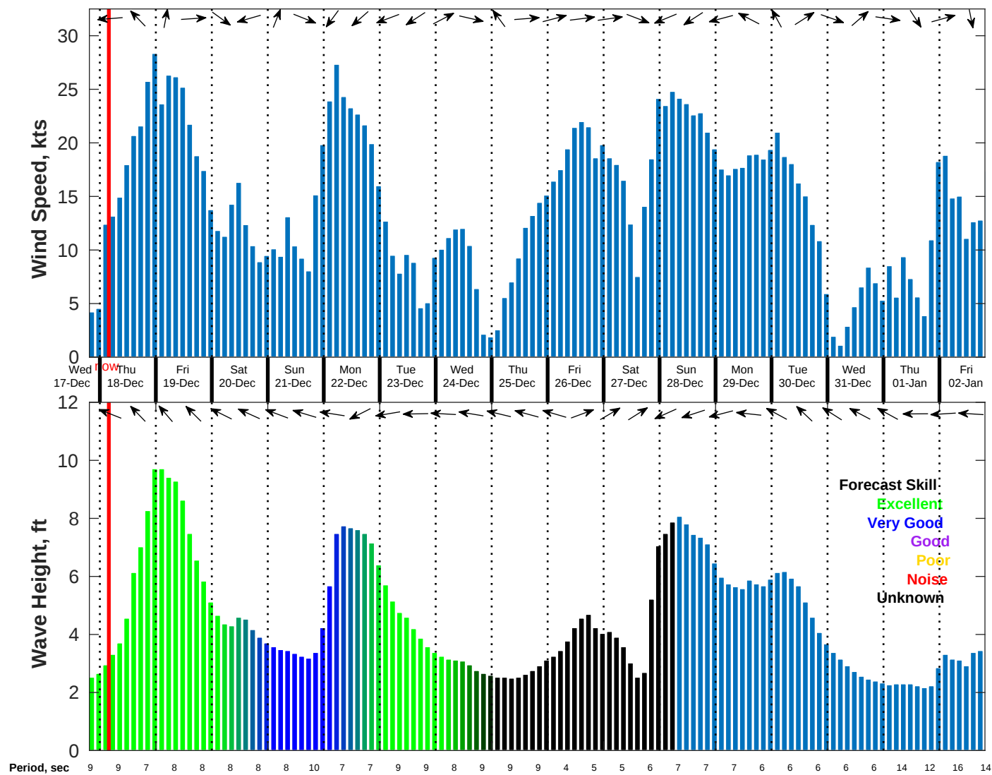
Wind & Wave Forecast for NDBC 41004 from 17-Dec-2025 19:00:00 to 02-Jan-2026 19:00:00
