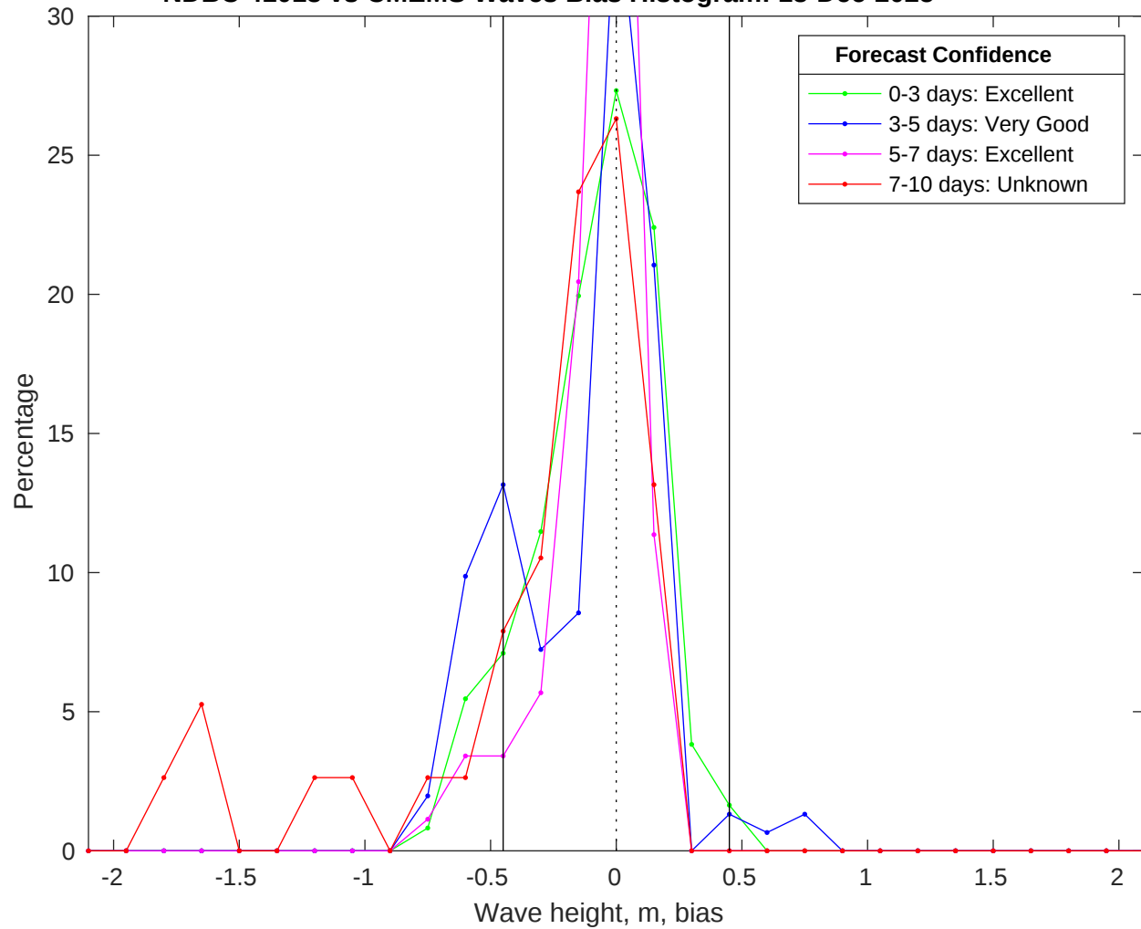
NDBC 41013 vs CMEMS Waves Bias Histogram: 18-Dec-2025
