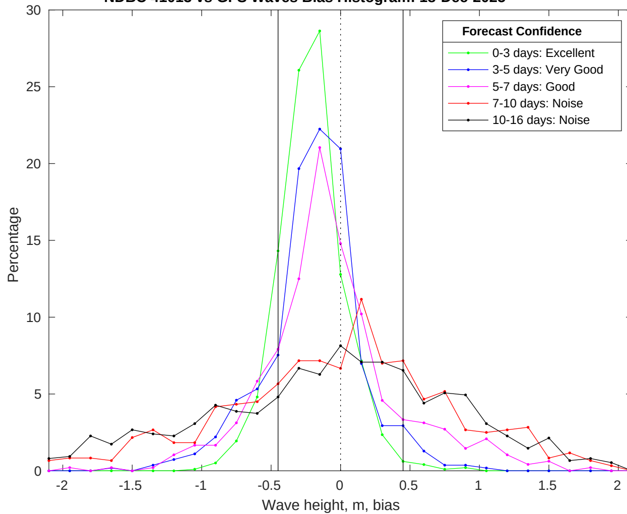
NDBC 41013 vs GFS Waves Bias Histogram: 18-Dec-2025
