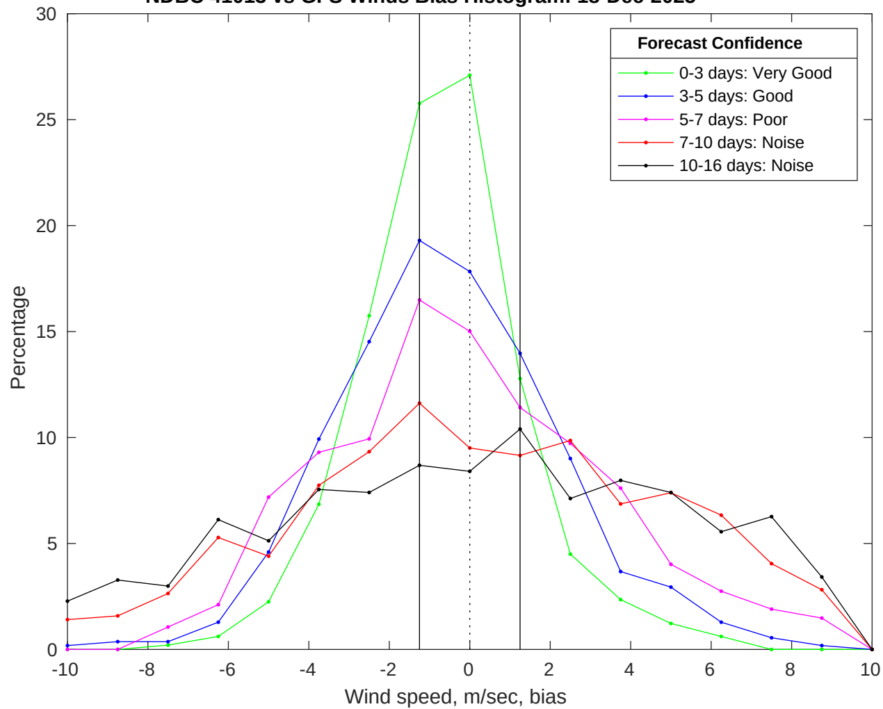
NDBC 41013 vs GFS Winds Bias Histogram: 18-Dec-2025
