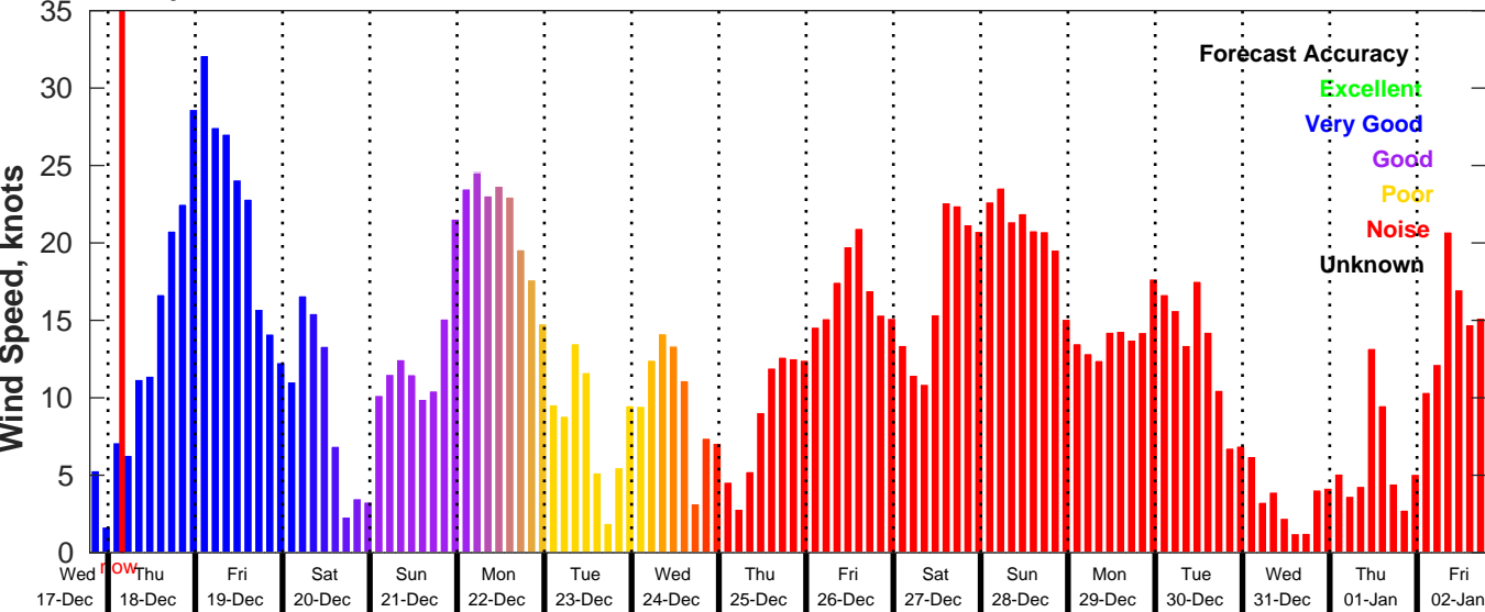
GFS Wind Speed Forecast for NDBC 41013 from 17-Dec-2025 19:00:00 to 02-Jan-2026 19:00:00
