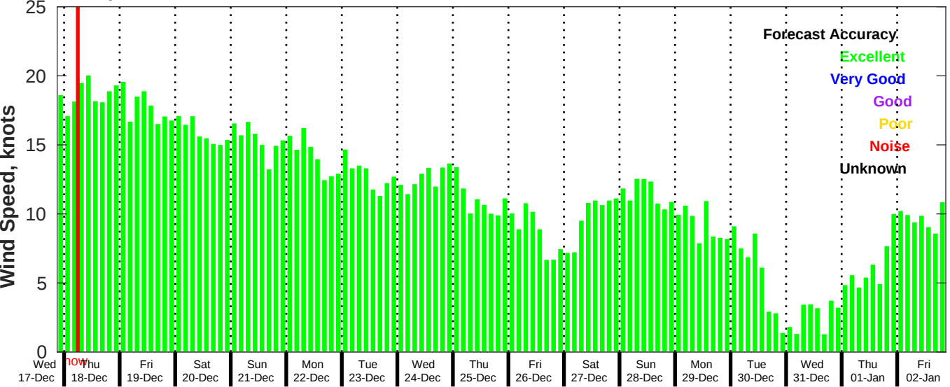
GFS Wind Speed Forecast for NDBC 41040 from 17-Dec-2025 21:00:00 to 02-Jan-2026 21:00:00
