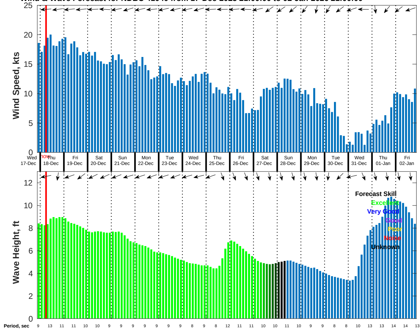
Wind & Wave Forecast for NDBC 41040 from 17-Dec-2025 21:00:00 to 02-Jan-2026 21:00:00
