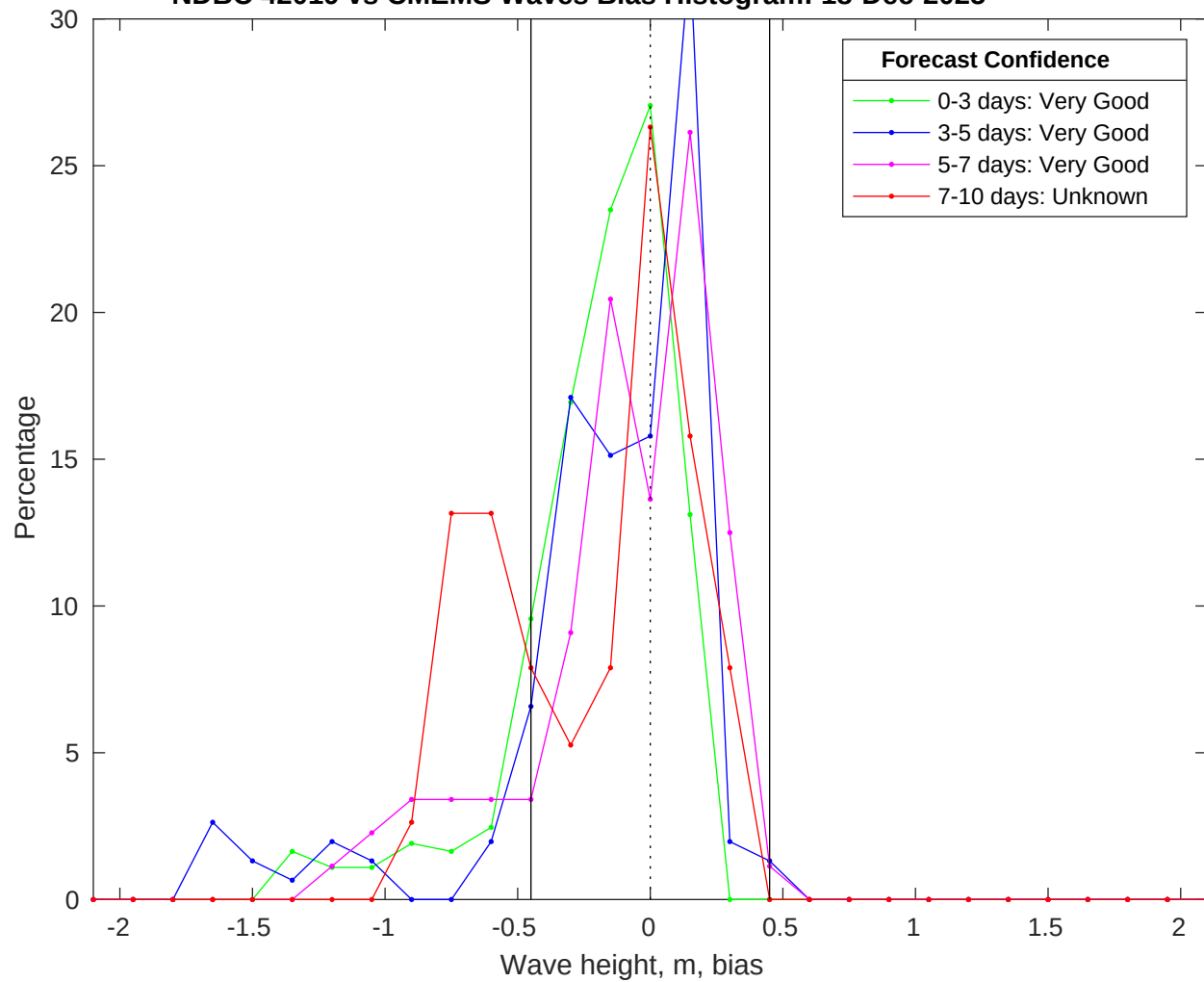
NDBC 42019 vs CMEMS Waves Bias Histogram: 18-Dec-2025
